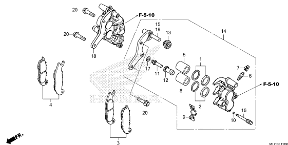
REAR BRAKE CALIPER
