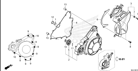
GENERATOR COVER/LEFT REAR COVER
