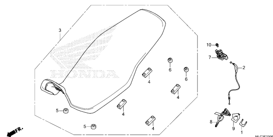
SEAT
