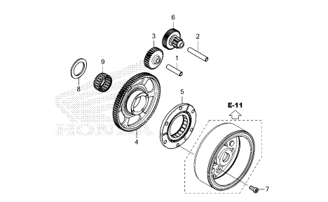
STARTING CLUTCH
