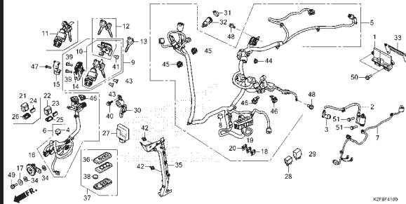
F-41 WIRE HARNESS (ACF110CBTM/N-IN,3IN)
