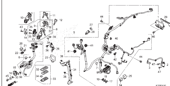
F-41-2 WIRE HARNESS (ACF110CBTP-IN,3IN)
