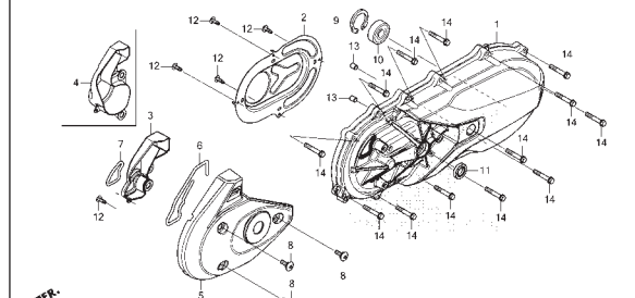
E-13 LEFT CRANKCASE COVER
