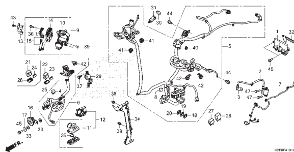
F-41-1 WIRE HARNESS (ACF110CBTM/N-2IN,4IN)
