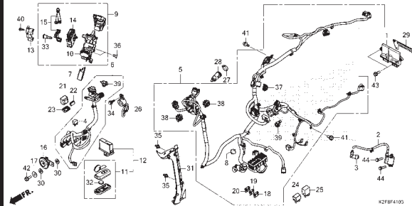
F-41-3 WIRE HARNESS (ACF110CBTP-2IN,4IN)
