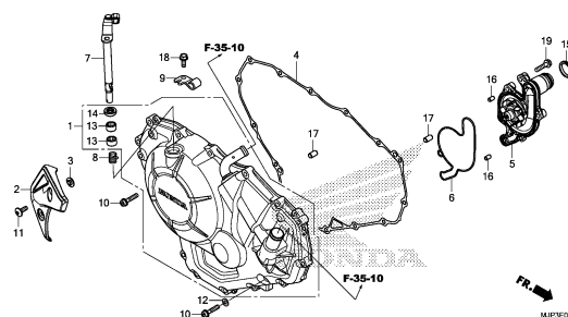
RIGHT CRANKCASE COVER (CRF1000/CRF1000A)
