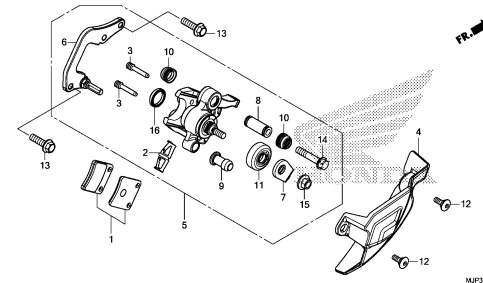
PARKING BRAKE CALIPER
