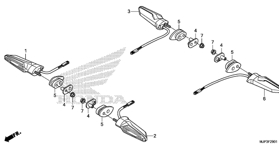
WINKER(CRF1000A/CRF1000D)
