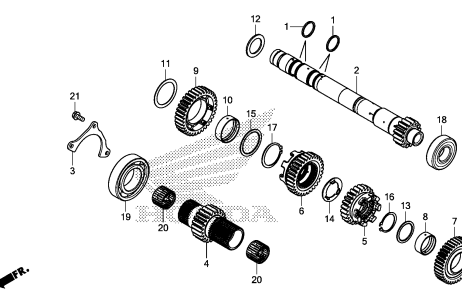
TRANSMISSION(MAINSHAFT)(CRF1000D)
