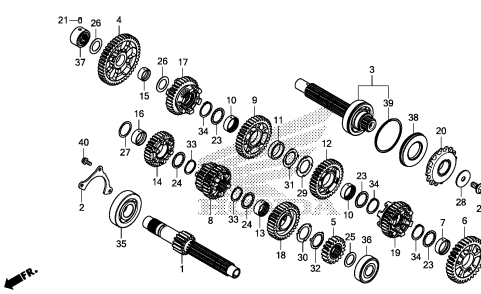
TRANSMISSION(CRF1000/CRF1000A)
