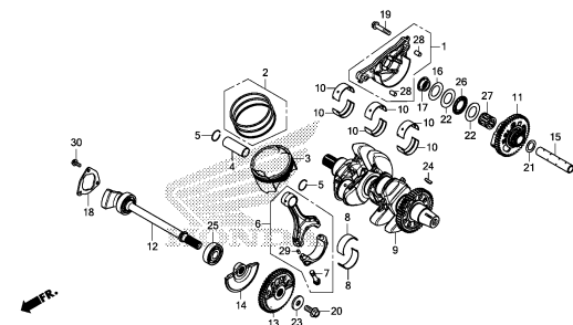
CRANKSHAFT/PISTON
