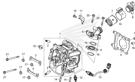
CYLINDER
