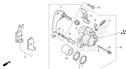
FRONT BRAKE CALIPER
