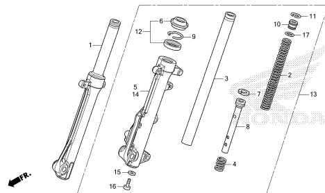
FRONT FORK
