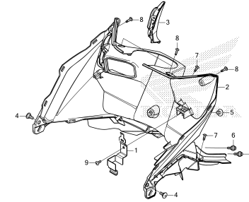
BODY COVER
